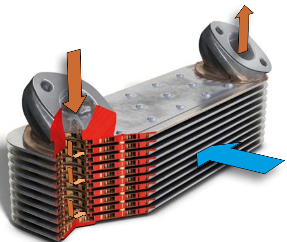
Oil cooler in a utility vehicle
